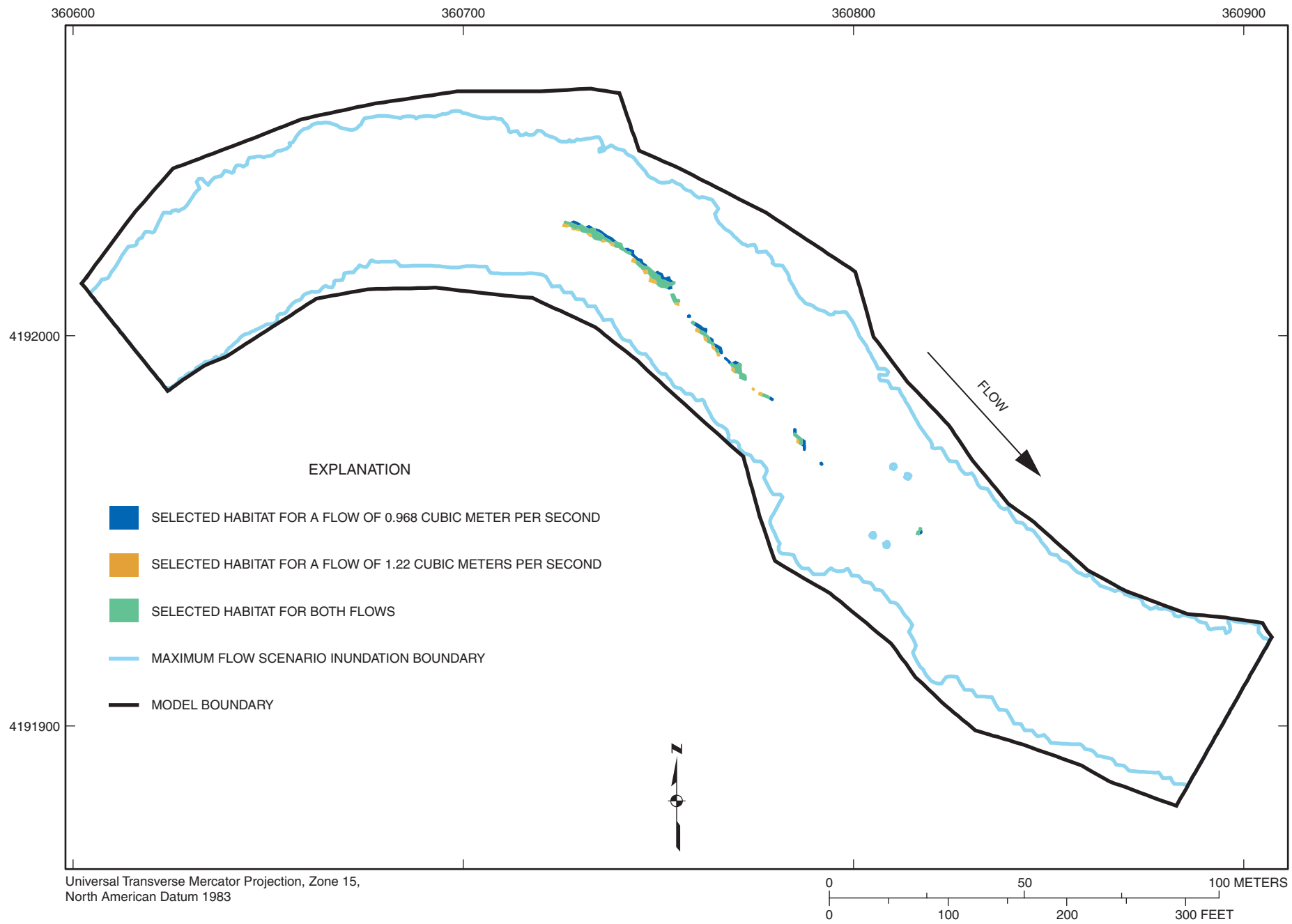
Figure 1-50. Selected habitat area distribution for habitat category 22 (channel catfish) at flows of 0.968 and 1.22 cubic meters per second at Marmaton River site M1.
